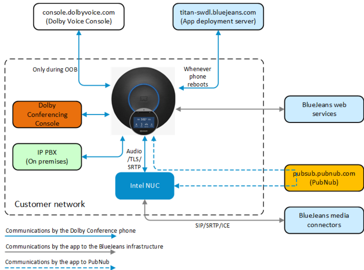
Figure 2: BlueJeans local setup architecture
